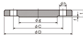
BL-RF
