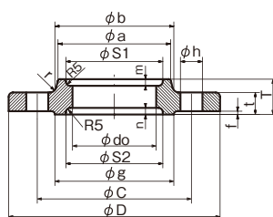
SOH-RF (B 形)
