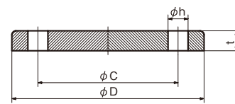
BL-FF
