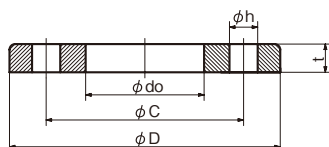
SOP-FF
