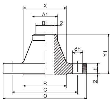
WN-RF
