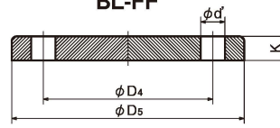
BL-FF
