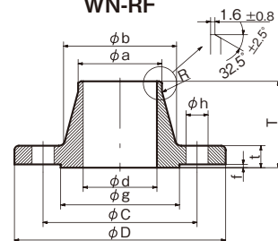
WN-RF
