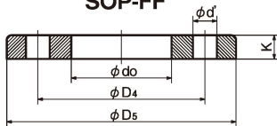
SOP-FF
