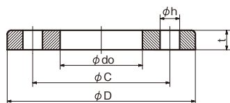
SOP-FF
