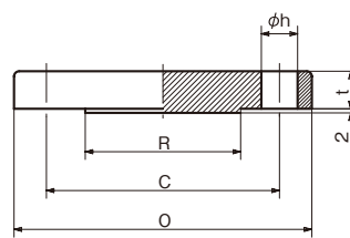
BL-RF
