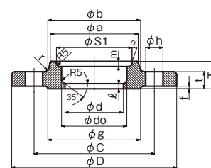
SOH-RF (C 形)
