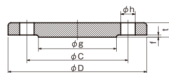
BL-RF
