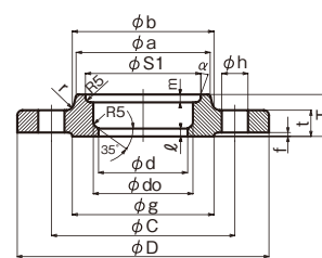
SOH-RF (C 形)
