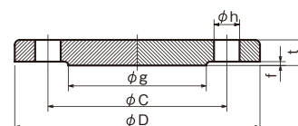
BL-RF
