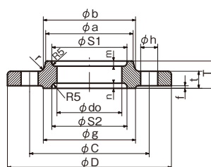
SOH-RF (B 形)
