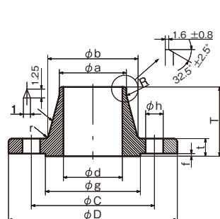
WN-RF
