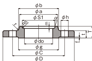
SOH-RF (A 形)
