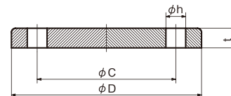
BL-FF
