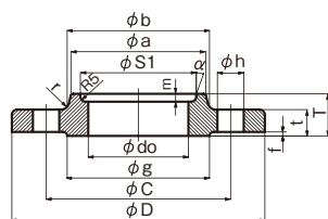
SOH-RF (A 形)
